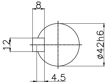
OUTPUT SHAFT
